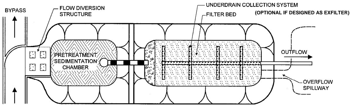
PLAN VIEW
