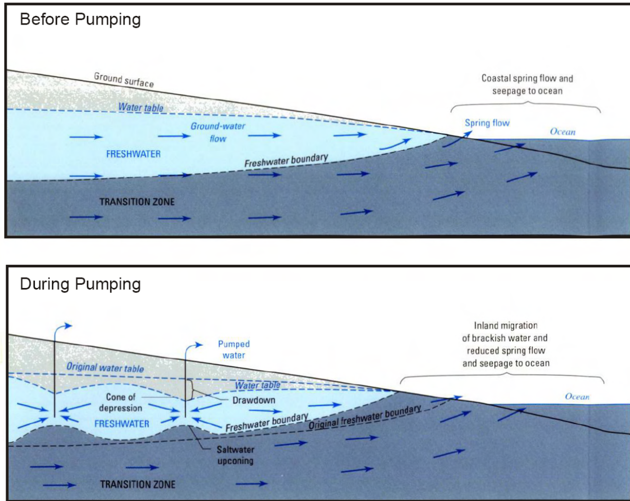
Figure 1.11 Effects of ground-water withdrawal on the potable part of the freshwater lens in a high permeability island aquifer. (Source: USGS Robert L. Carruth)
