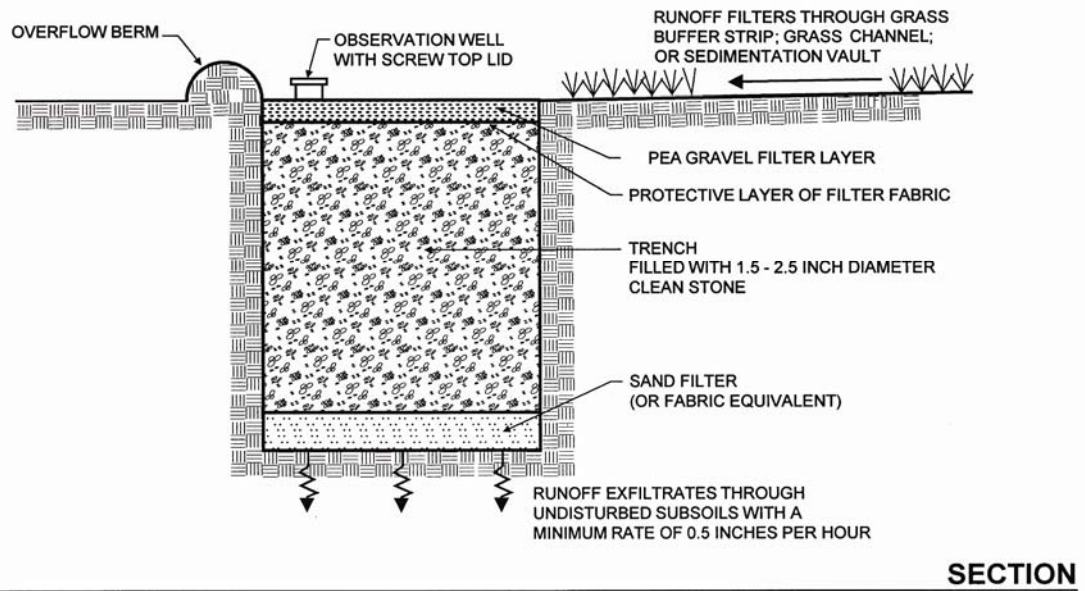
Figure 3.8 Infiltration Trench/Chamber (I-1)
