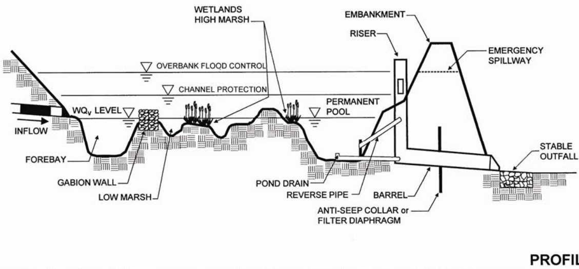
Figure 3.5 Shallow Marsh (W-1)
