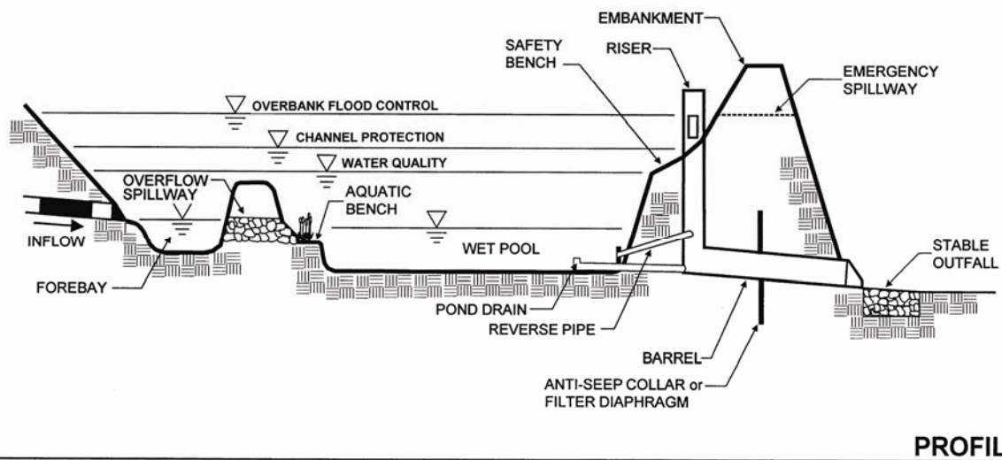
Figure 3.3 Wet Extended Detention Pond (P-3)
