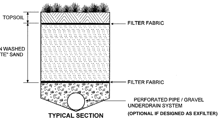
TYPICAL SECTION
