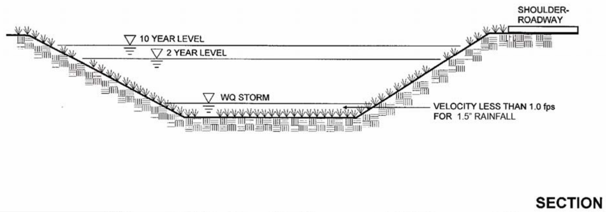
Figure 3.18 Grass Channel (LA-4)
