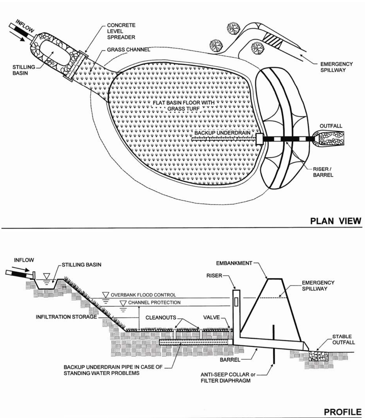
Figure 3.9 Infiltration Basin (I-2)
