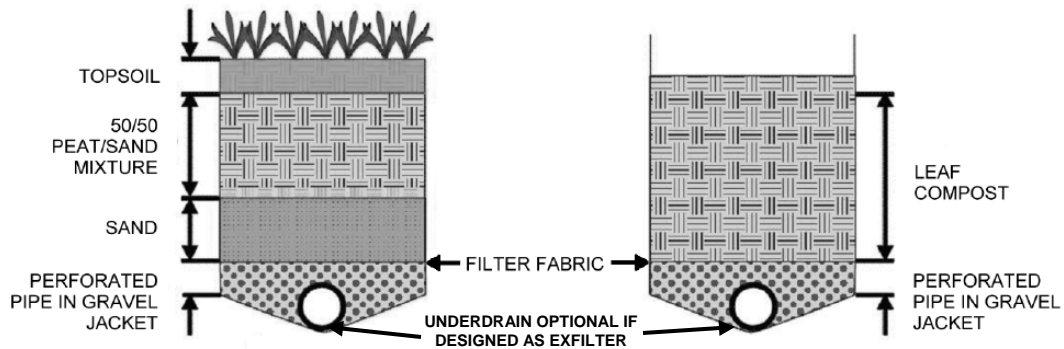
TYPICAL SECTIONS
