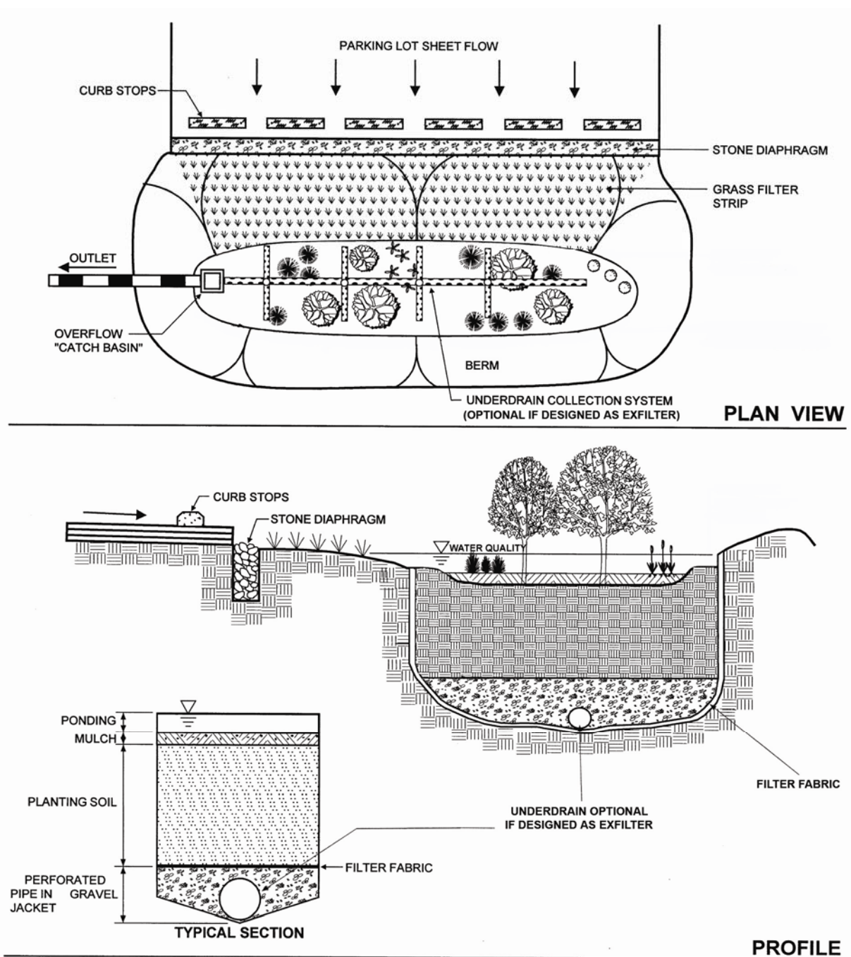
Figure 3.12 Bioretention (F-3)
